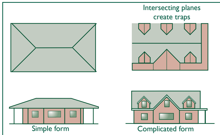
Roof forms
